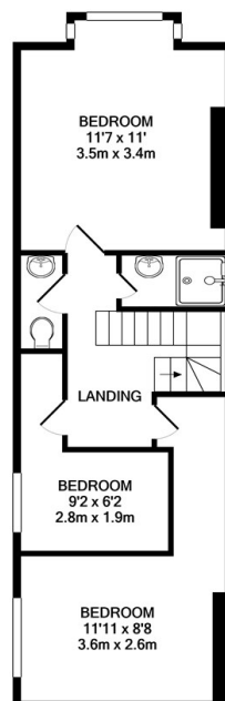
2ND FLOOR
